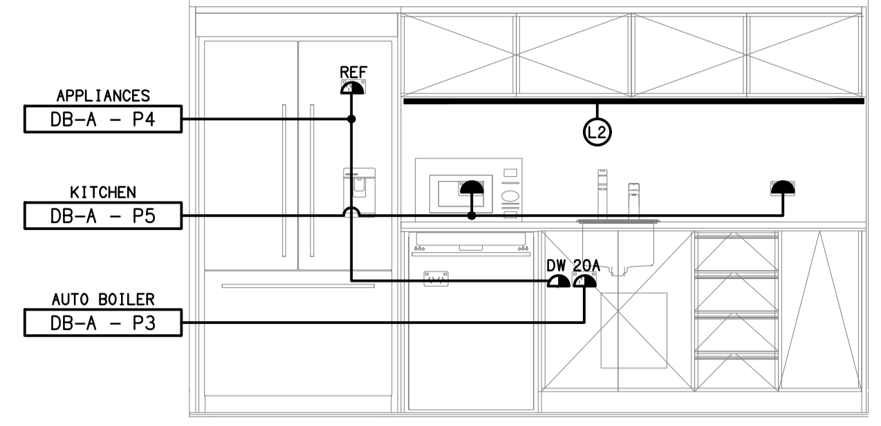
DETAIL A STAFF KITCHENETTE ELEVATION NOT TO SCALE
