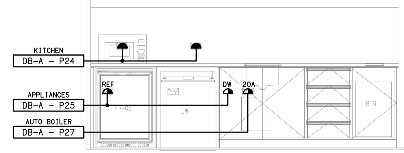
DETAIL C SHOWROOM KITCHENETTE ELEVATION NOT TO SCALE
