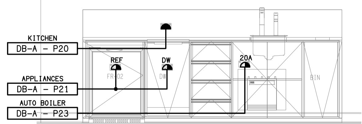
DETAIL B LOUNGE KITCHENETTE ELEVATION NOT TO SCALE
